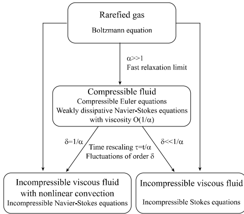
Figure 2. Hydrodynamic limits of the Boltzmann equation
