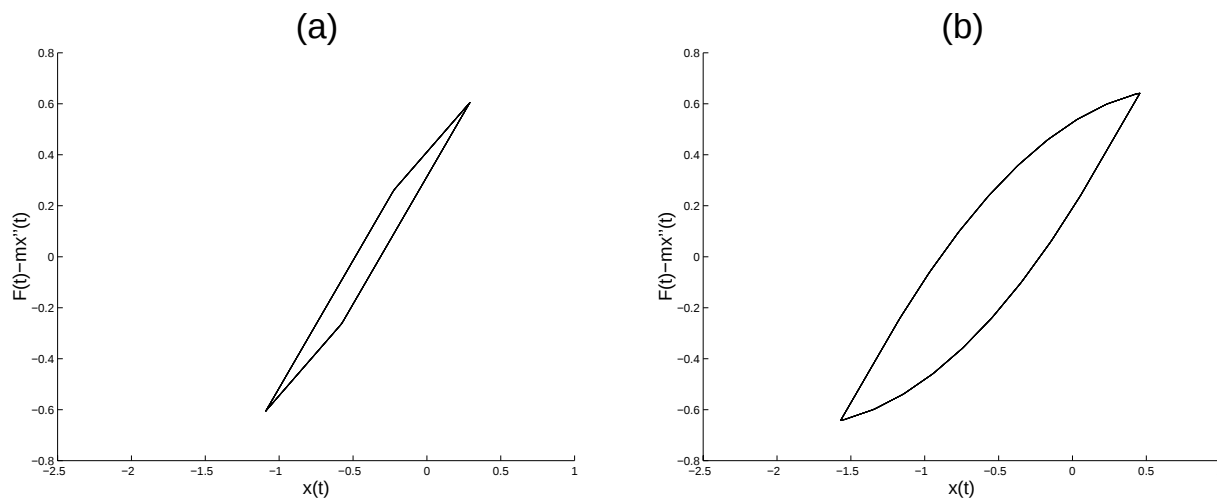
FIGURE 3. Curves \{x(t), F(t) - m\ddot{x}(t)\}_{400 \leq t \leq 500} for n = 3 (a) and n = 10 (b).
