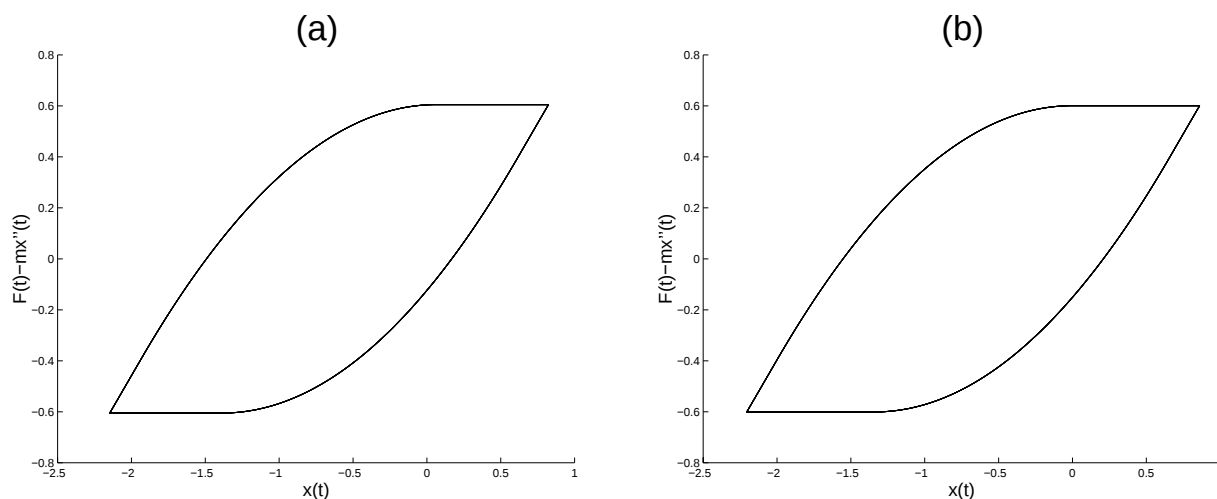
FIGURE 4. Curves \{x(t), F(t) - m\ddot{x}(t)\}_{400 \leq t \leq 500} for n = 100 (a) and n = 700 (b).
